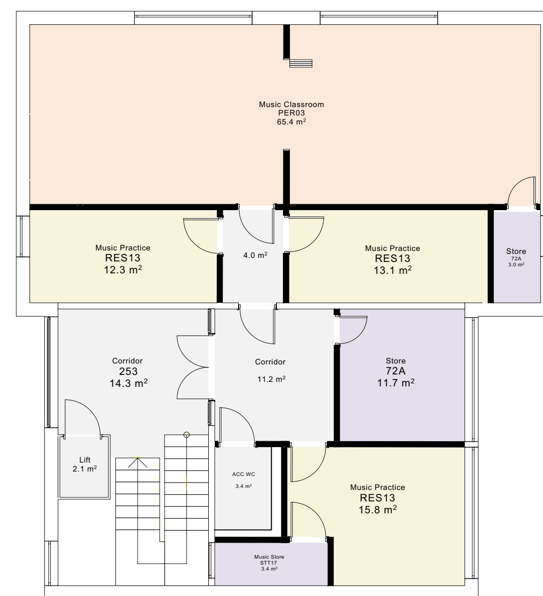
Proposed First Floor Plan - NTS
