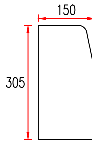
HALF BATTERED KERB (HB1) (K9)
