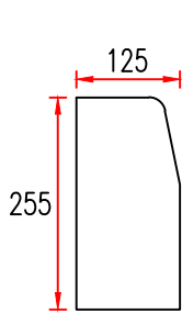
HALF BATTERED KERB (HB2) (K1-K5)
