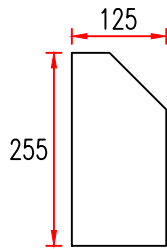
SPLAYED KERB (SP) (K7)
