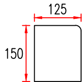
BULLNOSED KERB (BN) (BK8)
