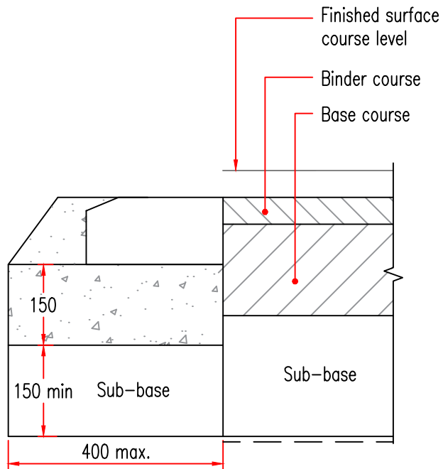
TEMPORARY KERB TYPE HB LAID ON BACK
