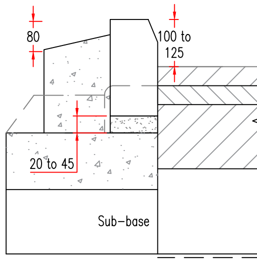
RAISE NEW KERB ON EXISTING BED & MORTAR
