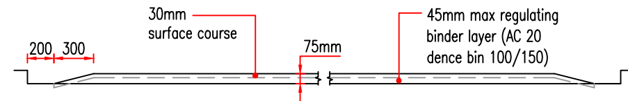
SECTION B-B
