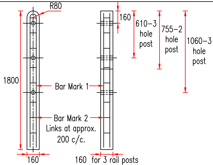
CONCRETE POST 2 & 3 RAIL
