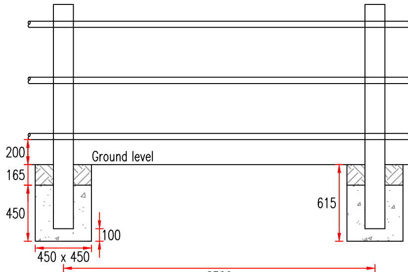
FOOTING DETAIL
